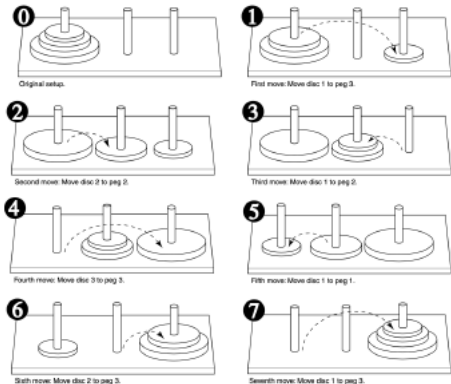
Figure 9: Recursion
